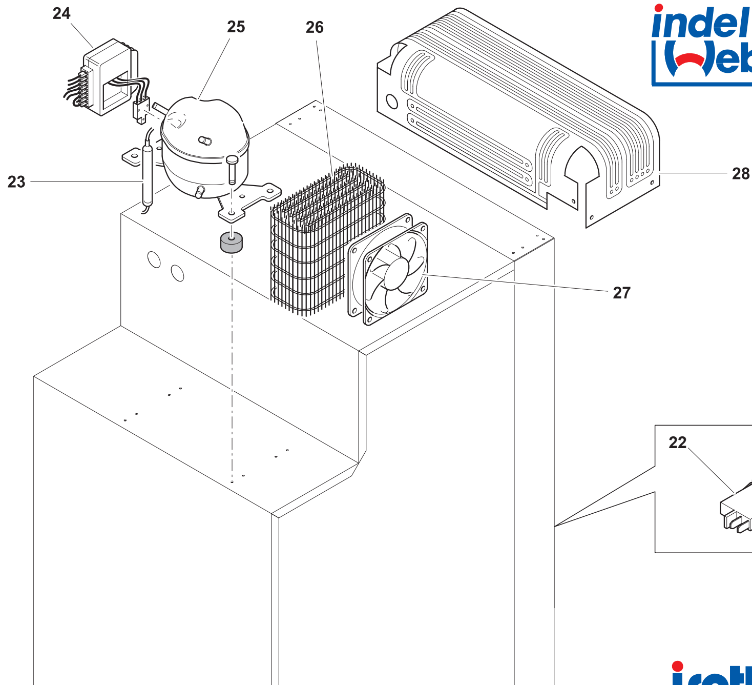
DR 130 INOX - COOLING UNIT
