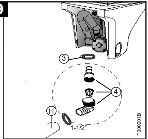
Horizontal Installation
