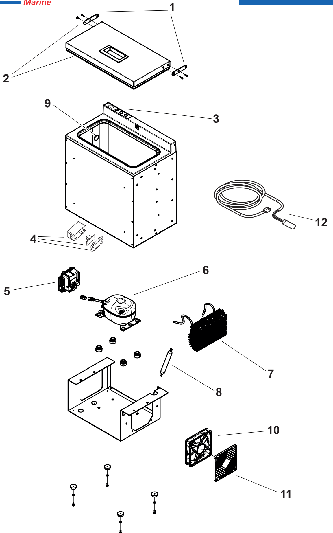
BUILT-IN 16 - CABINET & COOLING UNIT
