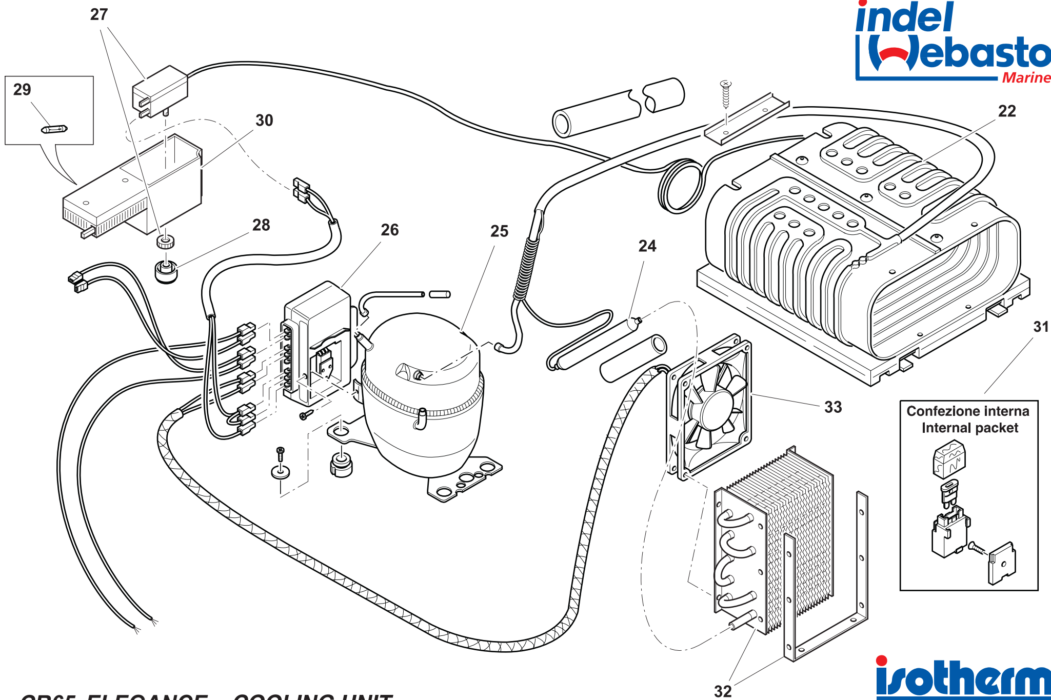
CR65 ELEGANCE - COOLING UNIT
